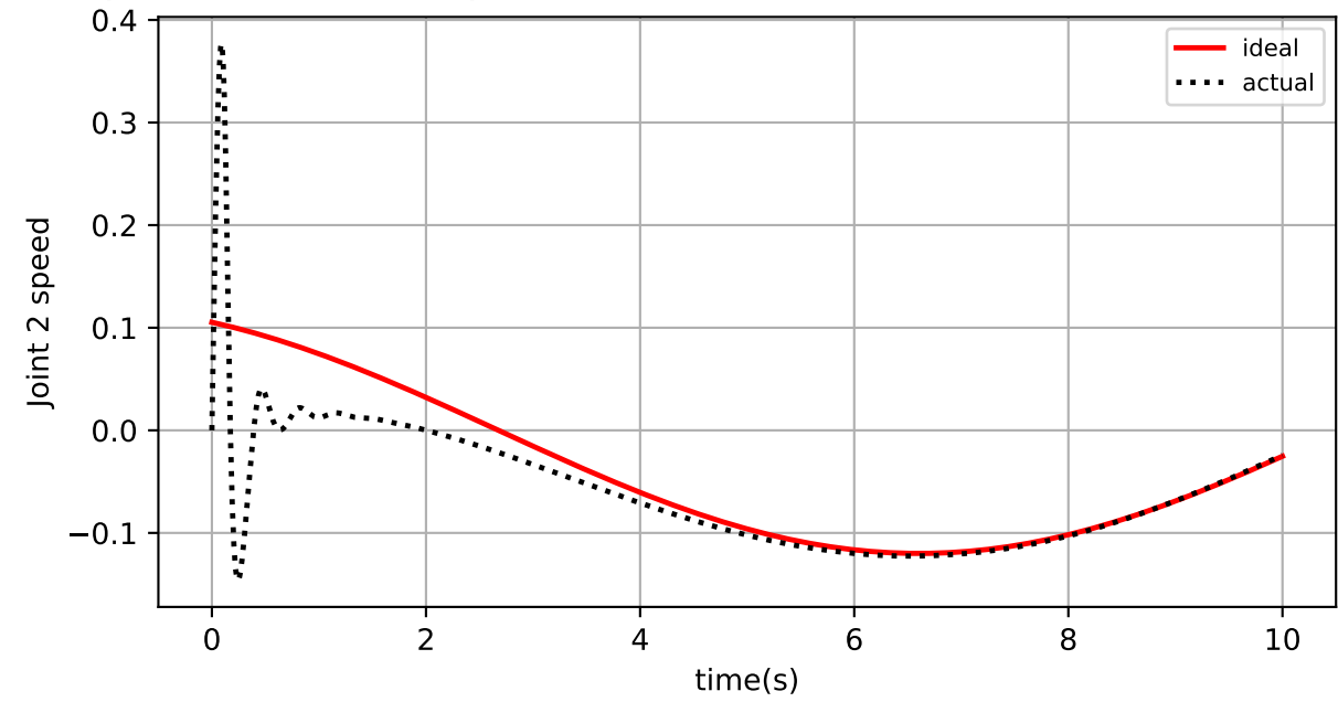
Speed Tracking Performance ( S=3 , S1=2 , m=5 )
